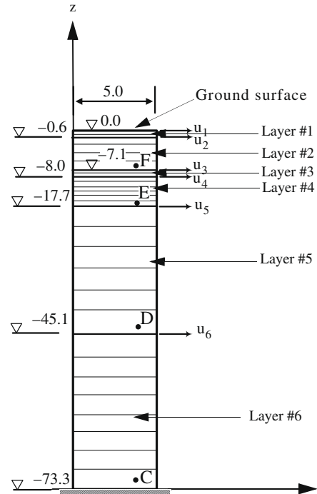
Fig. 12. Layered soil column subjected to total base acceleration with finite element mesh in thin lines (unit: [m]). Soil layers are numbered from top to bottom.
