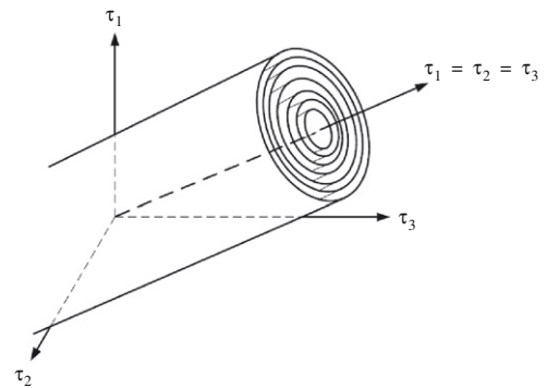
(b) Von Mises multi-yield surfaces
