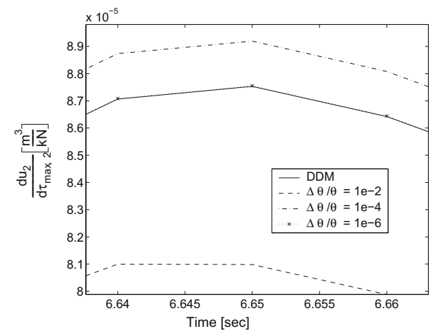
Fig. 21. Sensitivity of displacement response u_2 (see Fig. 12) to shear strength \tau_{\max,2} obtained using DDM and FFD with increasingly small perturbations of sensitivity parameter (zoom view of Fig. 20).
