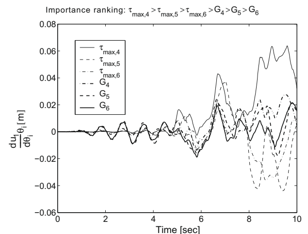
Fig. 22. Relative importance of material parameters on horizontal displacement response of ground surface (top of soil column, see Fig. 12).
