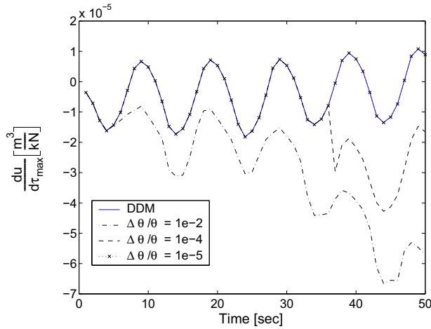
Fig. 11. Sensitivity of displacement response u(t) of node A in the x_1 -direction to the shear strength \tau_{\max} computed using DDM and FFD for three different values of relative parameter perturbation \Delta\theta/\theta .
