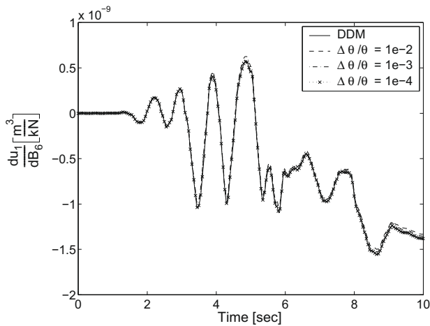
Fig. 18. Sensitivity of displacement response u_1 (see Fig. 12) to bulk modulus B_6 obtained using DDM and FFD with increasingly small perturbations of sensitivity parameter.
