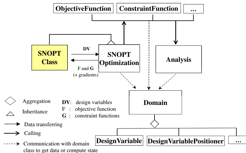
Fig. 3. SNOPT-based optimization used for model updating or structural optimization/identification
